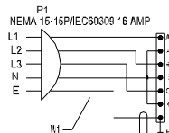
380V-415 VAC 3 PHASE WYE
